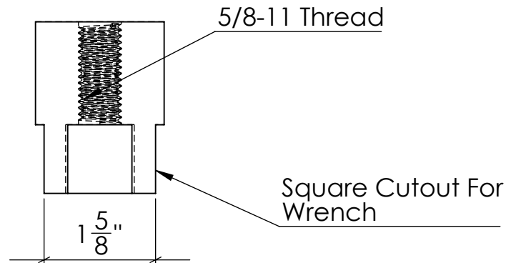
Thread Insert For Bottom Plate
