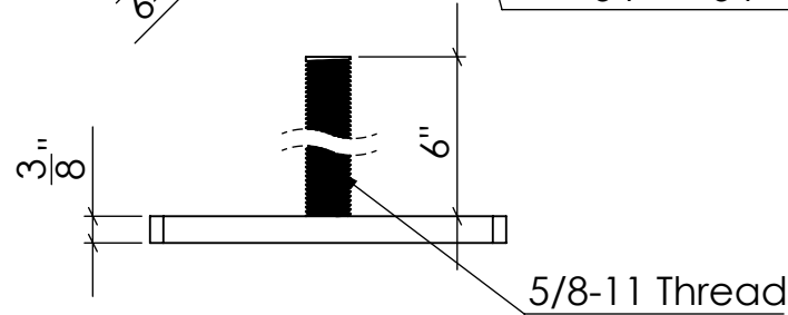
Base Plate Details
